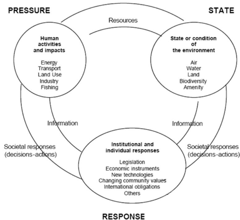
Figure 1: Pressure State Response model diagram (Quality Planning 2009)
